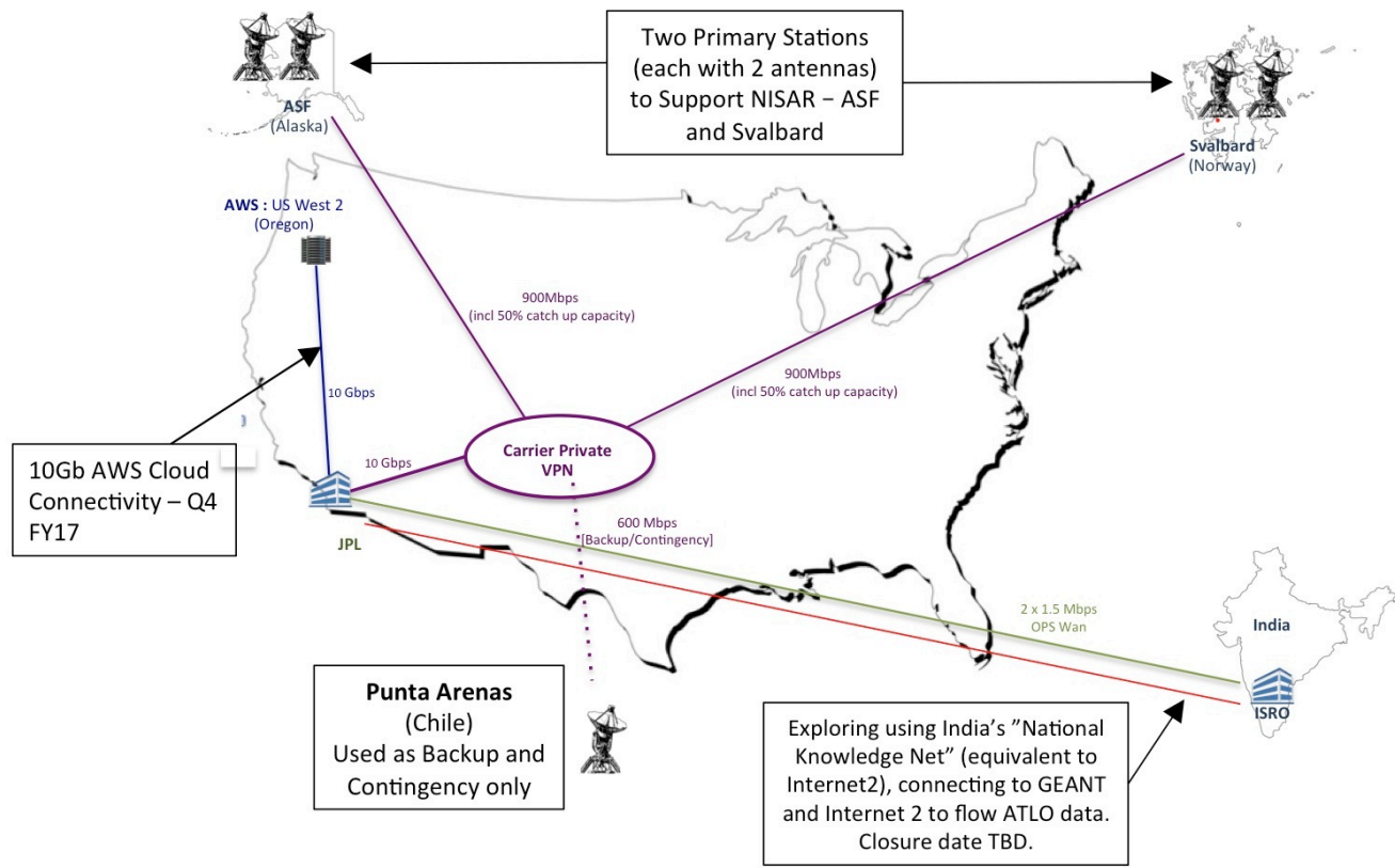
Figure 3 – Current ground station network envisioned for NISAR. Data transfer between the downlink stations and the processing centers is also shown. Processing will be done at ISRO and at a center in Oregon, with U.S. transfer funneling through JPL.
